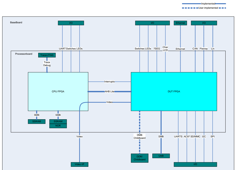
MPB-M3 Block Diagram I/O
